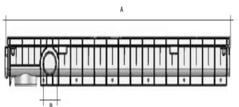
Vista laterale Side view
